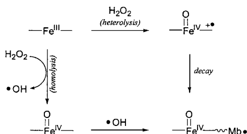
FIG. 4. Heterolytic and hemolytic pathways of peroxide cleavage by myoglobin. (modified from Ref. 198).
