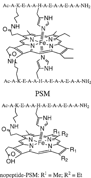
FIG. 3. Chemical structures of (top) the peptide sandwiched mesoheme (PSM) and (bottom) its mono-peptide analog. Reprinted with permission from Ref. (108). Copyright 1995 American Chemical Society.
