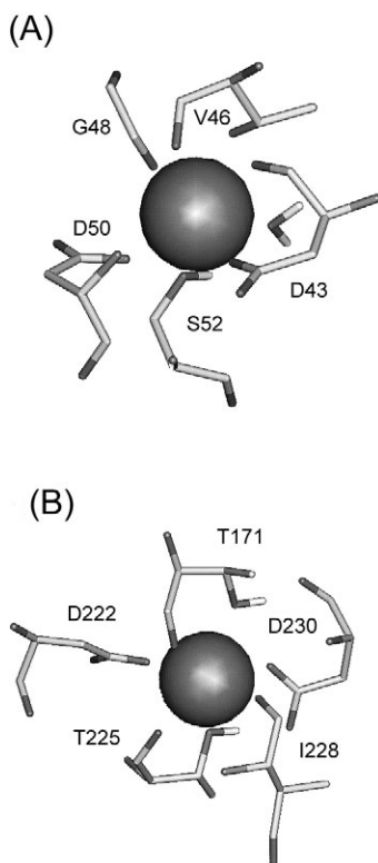
FIG. 7. The calcium binding sites of HRP C (detail). Ligands to the distal (A) and proximal (B) calcium atoms are shown. The O-donor ligand sets are listed in Section IV,D.
