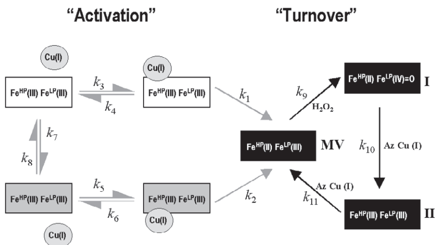
FIG. 10. A model of the mechanism of activation and turnover in P. aeruginosa CCP after Foote et al. (62). In order to successfully model steady-state turnover, Foote et al. used the following experimentally derived rate constants: k_1 = 7 \text{ s}^{-1} , k_2 = 0.2 \text{ s}^{-1} , k_9 = 5.6 \times 10^7 \text{ M}^{-1}\text{s}^{-1} , k_{10} = 2.0 \times 10^6 \text{ M}^{-1}\text{s}^{-1} , k_{11} = 1.5 \times 10^6 \text{ M}^{-1}\text{s}^{-1} (62). In addition the following rate constants were determined by kinetic modeling; k_3 = 5 \times 10^4 \text{ M}^{-1}\text{s}^{-1} , k_4 = 3.4 \text{ s}^{-1} , k_5 = 1 \times 10^6 \text{ M}^{-1}\text{s}^{-1} , k_6 = 4.2 \text{ s}^{-1} , k_7 = 0.125 \text{ s}^{-1} , k_8 = 0.1 \text{ s}^{-1} (62). Note that the origin of the equilibrium ( k_7/k_8 ) between conformers of CCP that gives rise to the fast phase of activation (white infilled rectangles) and that giving rise to the slow phase of activation (gray infilled rectangles) is unknown. If, however, it arises from \text{Ca}^{2+} binding to the enzyme, a more complex model would be required, as presumably an equilibrium would exist between catalytically active ( \text{Ca}^{2+} bound) and inactive ( \text{Ca}^{2+} free) states of the MV state. Such models have been put forward for the P. denitrificans CCP by Prazeres et al. (17) and Lopes et al. (16).
