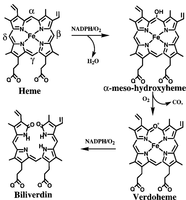
FIG. 15. Overall reaction catalyzed by heme oxygenase.
