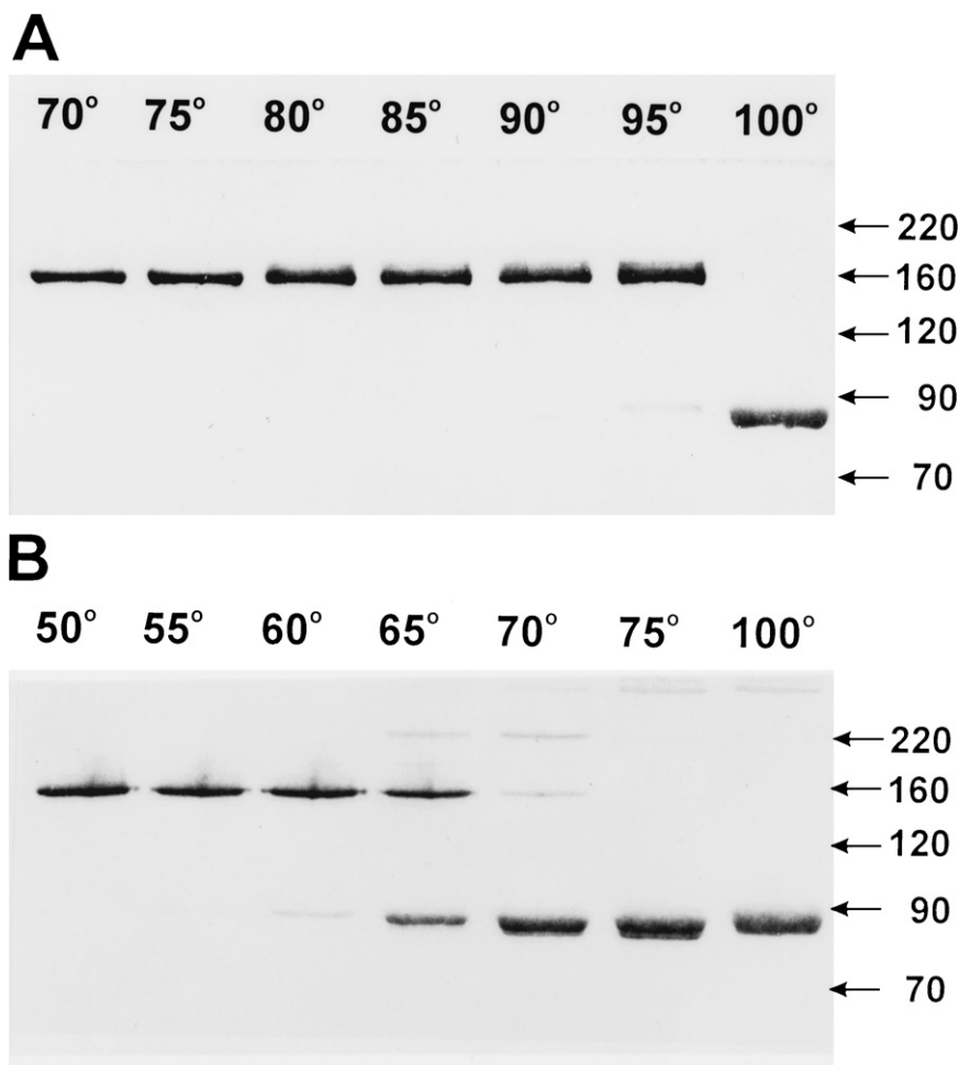
FIG. 11. Conversion of HP11 dimers to monomers. In panel A , HP11 was incubated for 10 min at 70, 75, 80, 85, 90, 95, and 100°C in 50 mM potassium phosphate buffer (pH 7). In panel B , HP11 was incubated for 10 min at 50, 55, 60, 65, 70, 75, and 100°C in 50 mM potassium phosphate (pH 7) and 5.6 M urea. The temperatures of incubation are indicated above each lane. In both panels A and B , samples were removed, cooled to room temperature, and added to SDS-urea loading buffer. Samples were loaded and run, without further heating, on an 8% polyacrylamide gel. Reprinted with permission from Switala et al. (86). Copyright 1999 American Chemical Society.
