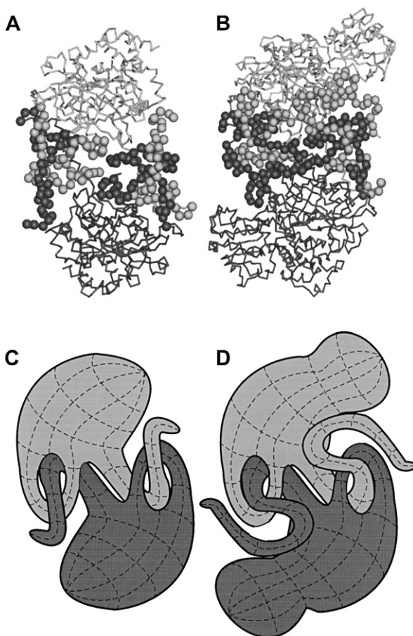
FIG. 10. Illustration of the interweaving of two subunits of the small-subunit BLC ( A ) and the large-subunit HP11 ( B ). The residues in the immediate proximity of the overlaps are shown as spheres. A schematic representation of the interwoven structures are shown in C for BLC and D for HP11. Note the longer N-terminal region of HP11 (80 residues in HP11 as compared to 25 in BLC) that extend through the loop on the opposite subunit.
