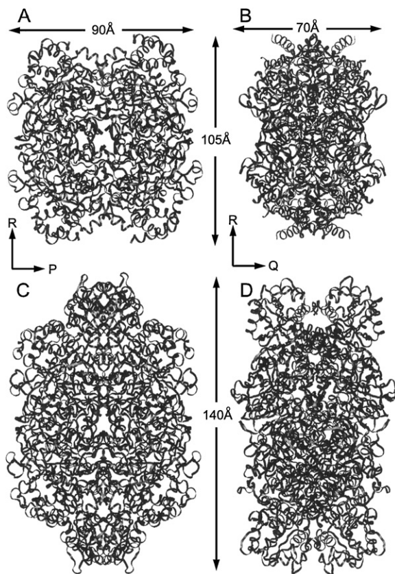
FIG. 9. Comparison of the dimensions of small-subunit (BLC) and large-subunit (HPII) catalases. BLC is shown in panels A and B , in the R - P and R - Q orientations, respectively; HPII is shown in C and D , also in the R - P and R - Q orientations, respectively.
