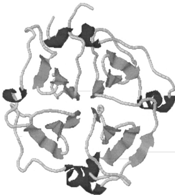
FIG. 7. The crystal structure of the C-domain of hemopexin (PDB accession number 1HXN) (128) showed a four-bladed \beta -propeller structure, which because of sequence similarity was also expected in the N-domain. The high degree of beta structure and limited \alpha -helix content agrees with the earlier FTIR analysis.
