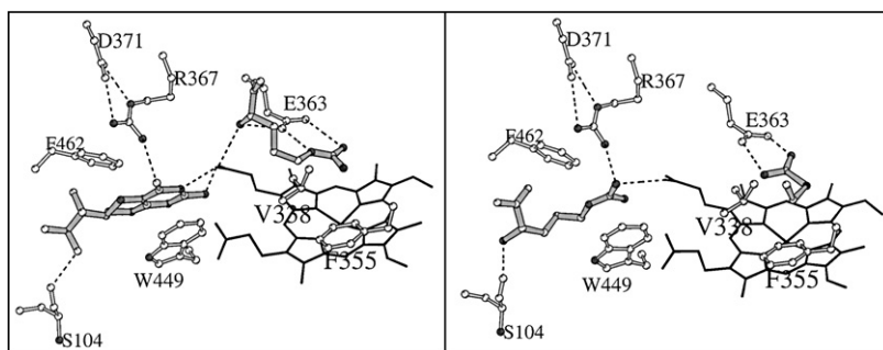
FIG. 8. Comparison of the pterin-bound and -free structures. In the absence of pterin with the SEITU inhibitor in the active site (right), L-Arg binds in the pterin site. L-Arg is an excellent mimic for H 4 B owing to the similar H-bonding pattern with the heme propionate and Ser104, and the ability of the L-Arg guanidinium group to aromatically stack with Trp449.
