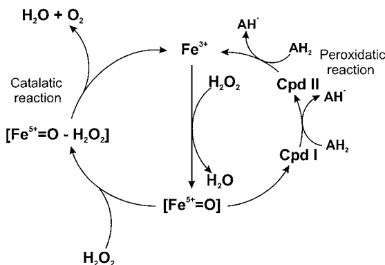
FIG. 7. Catalytic and peroxidatic reactions of type B enzymes. This represents a modification of the schemes of Figs. 2 and 5A and is proposed to account for the characteristic features of catalase-peroxidases. Compound I is drawn as \text{Fe}^{5+}=\text{O} and can represent either a \pi -cation radical or alternative radical structure. The precise nature remains undefined (see Section IV,F).
