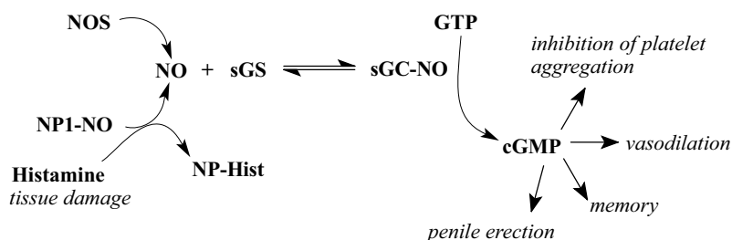
FIG. 1. Nitric oxide (NO) synthesis by nitric oxide synthase (NOS) (upper left), NO reaction with soluble guanylate cyclase (sGC) (middle), and formation of cyclic GMP, which causes tissue-specific signaling (right). The roles of the salivary nitrophorins from Rhodnius prolixus in storing and releasing NO and binding histamine are included (lower left).
