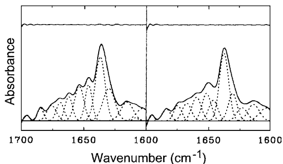
FIG. 6. Deconvolved amide I' region FTIR spectra of apo- and heme-hemopexin. The amide I' FTIR spectra of apo- and heme-hemopexin in D_2O were recorded and curve-fitted to resolve the individual bands. The differences between the original and fitted curves are shown in the upper traces in the panels. The estimated helix (15%), beta (54%), turn (19%), and coil (12%) content of the apo-protein are not significantly changed upon heme binding (104). This analysis was required because of the positive 231-nm ellipticity band in hemopexin and is consistent with the derived crystal structure results.
