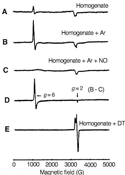
FIG. 3. EPR spectra of 100 pairs of Rhodnius salivary glands homogenized in 125 \mu l of phosphate-buffered saline at pH 7.2 (A) before argon equilibration; (B) after equilibration in an argon atmosphere for 4 h; (C) after equilibration of (B) with NO for 2 min. (D) difference spectrum, that is; B - C. (E) homogenate as in (B) treated with dithionite (DT) to reduce Fe(III) to Fe(II), followed by equilibration with NO for 2 min. (The small signal at g \approx 2 in A-C is due to copper oxide in the liquid helium which had been condensed at the University of Arizona in a copper-plumbed helium liquification apparatus!) All spectra are plotted on the same scale except (E), which is reduced in amplitude by a factor of 3. Reproduced with permission from Ref. (24).
