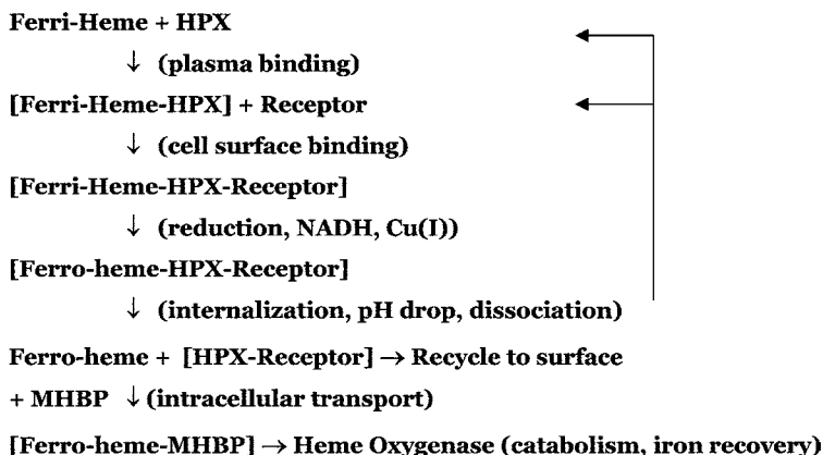
FIG. 17. Hemopexin-mediated heme transport. The following is a proposed scenario for the transport of iron-porphyrins by hemopexin. Evidence is cited throughout the text that supports the major features of this working model. However, questions remain, and the molecular details of several features will require further efforts to elucidate. The role of the hemopexin receptor in activating signaling pathways is presented elsewhere (89) and thus is not considered here.
