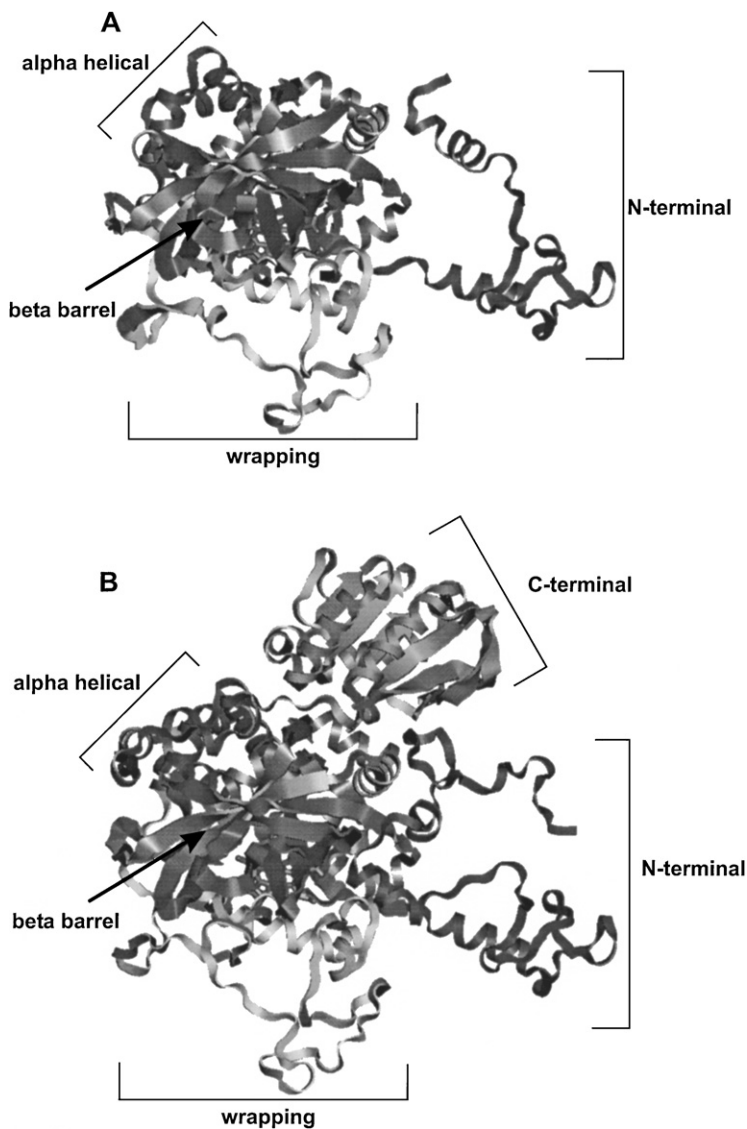
FIG. 8. Comparison of the subunit structures of a small subunit catalase (BLC) (A) and a large subunit catalase (HP11) (B). Segments including the N-terminal domain, the beta barrel core, the wrapping domain, the alpha helical domain, and the C-terminal domain (HP11) are indicated and are described in Section V,A.
