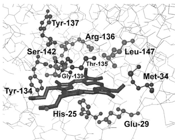
FIG. 7. Structure of the active site of truncated human HO-1 showing residues that are in the active site cavity (53).
