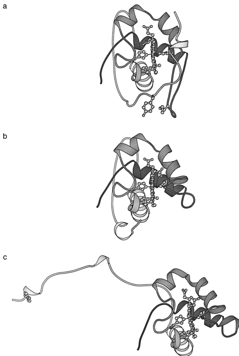
FIG. 5. The c -heme domain in cytochromes cd 1 from P. pantotrophus and P. aeruginosa . (a) Oxidised form of P. pantotrophus cytochrome cd 1 showing bis-histidine ligation of the heme iron. Tyr 25 that is a ligand to the d 1 heme can be seen at the bottom of the figure adjacent to Met 106. (b) Reduced form of P. pantotrophus cytochrome cd 1 showing the movement of Met106, which replaces His17 as a ligand. (c) Oxidized form of P. aeruginosa cytochrome cd 1 showing His/Met ligation coordination of the heme iron. To the left of the figure can be seen Tyr10, which is adjacent to the d 1 heme in the other subunit of the dimer. (Drawn from PDB entries 1 qks, 1 aof, and 1 nir.)
