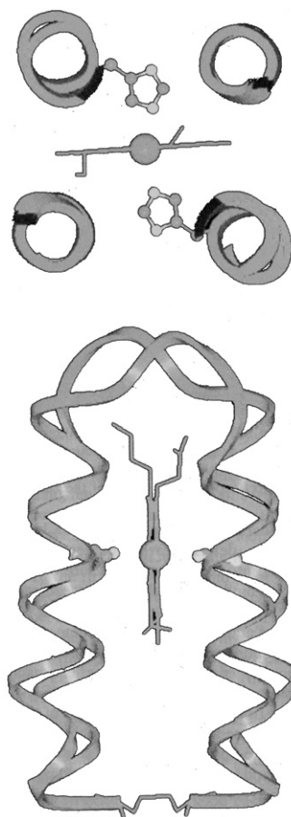
FIG. 5. Top and side view of a retro(S-S) molecular model containing heme. Reprinted with permission from Ref. (126). Copyright 1994 American Chemical Society.
