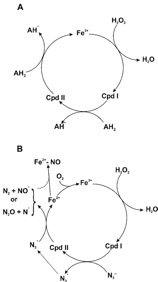
FIG. 5. (A) The peroxidatic reaction proceeding via compound II (the D2 family). (B) A catalytic cycle involving azide proceeding via compound II and ferroenzyme (the D5 family).
