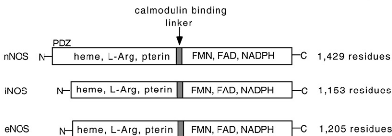
FIG. 1. The overall reaction catalyzed by NOS and a schematic representation of the three main NOS isoforms. L-Arg is first converted to N -hydroxy-L-Arg in a P450-like monooxygenation reaction requiring two electrons and one \text{O}_2 molecule. In the second step, N -hydroxy-L-Arg to NO and L-citrulline, only one electron and one \text{O}_2 molecule are required. nNOS, neuronal NOS (neural system); iNOS, inducible NOS (immune system); eNOS, endothelial NOS (cardiovascular system).
