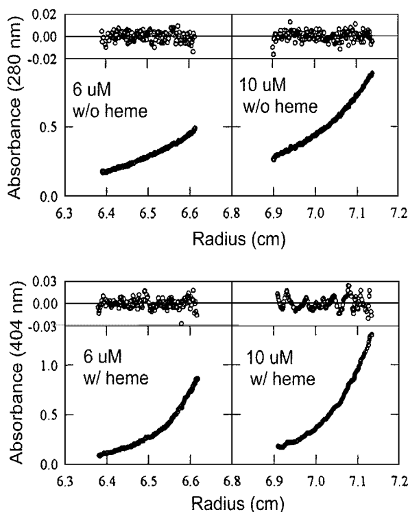
FIG. 5. Sedimentation equilibrium analysis of hemopexin domain interactions. Mixtures of N- and C-domain were centrifuged to equilibrium at 25°C in the absence (upper panels) and presence (lower panels) of heme. Nonlinear fitting procedures were performed to obtain apparent K_d values, and residuals of the fits are shown in the top portion of each panel (106).
