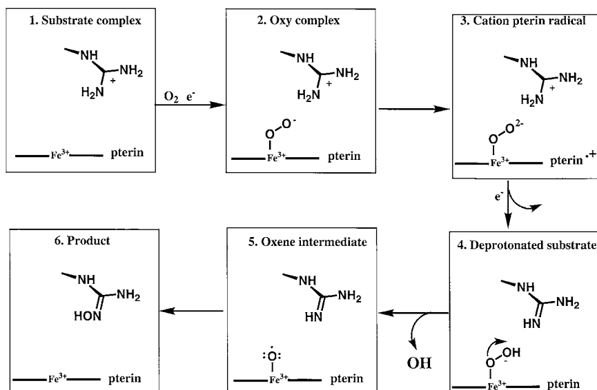
FIG. 9. Possible electron transfer mechanism for NOS utilizing a pterin radical. The oxy-complex in 2 is shown as the ferric ( \text{Fe}^{3+} )-superoxide complex. The role of the pterin then is to donate an electron to the iron, thus giving the peroxy dianion in 3 . The dianion is a potent base that abstracts a proton from the substrate, giving 4 . The system is now set up for a peroxidase-like heterolytic cleavage of the O-O bond to give the active hydroxylating intermediate in 5 and, finally, the first product in 6 .
