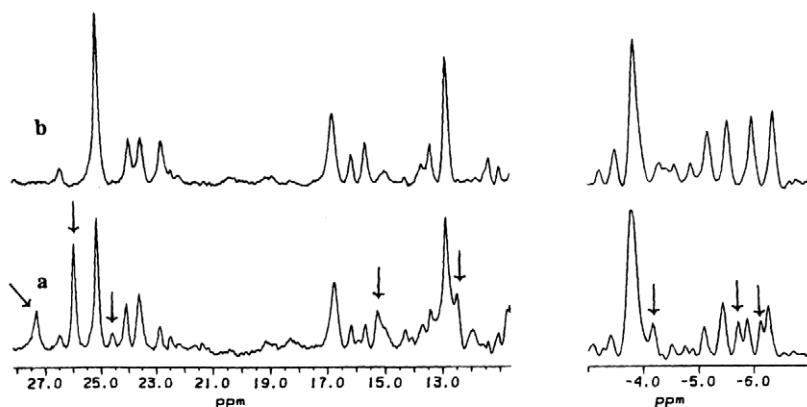
FIG. 11. 1D ^1\text{H} NMR spectrum of the hyperfine-shifted region of a sample of 4 mM NP1-ImH in \text{D}_2\text{O} at \text{pH}^* 7 (50 mM phosphate buffer) and 37^\circ\text{C} : (a) freshly prepared sample; (b) same sample 12 hours later. Reproduced with permission from Ref. (49).
