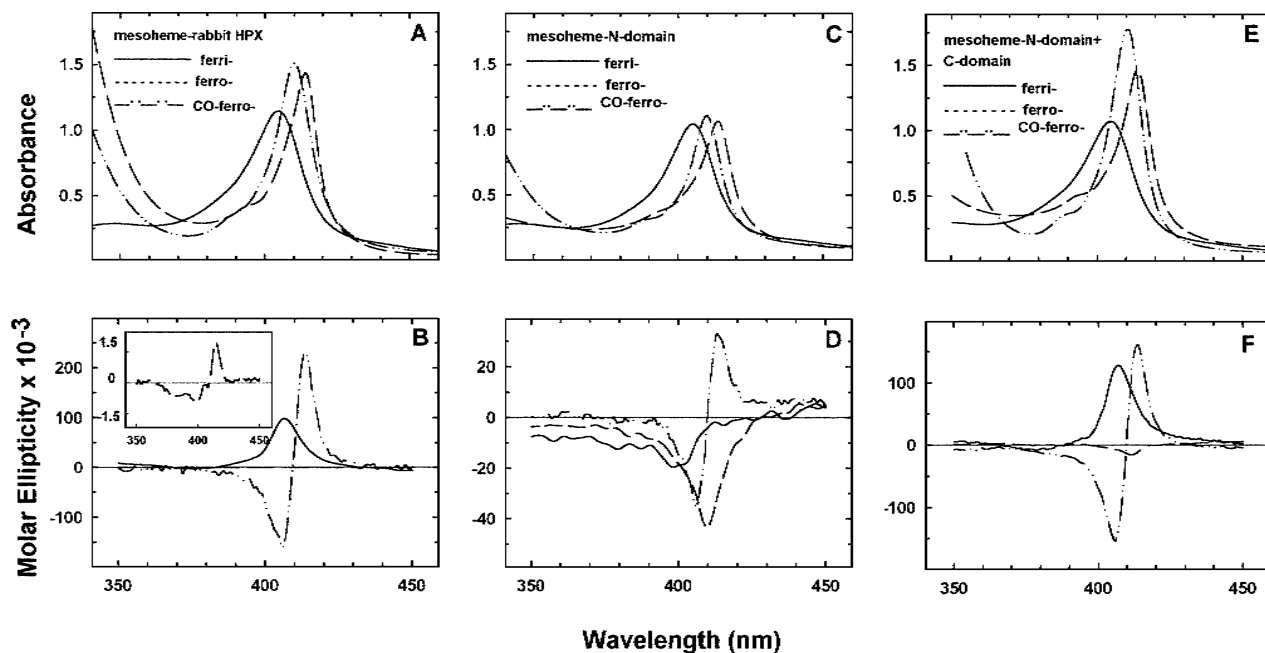
FIG. 11. Absorbance and CD spectra of ferri-, ferro-, and CO-ferro-heme complexes of hemopexin and its domains. Panels A, C, and E show the Soret region absorbance spectra, and panels B, D, and F the corresponding CD spectra. Rabbit hemopexin (panels A and B), N-domain (panels C and D), and N-domain–C-domain (panels E and F) complexes with mesoheme in the ferri- (solid lines), ferro- (dashed lines), and CO-ferro- (dash-double dot lines) states in phosphate-buffered saline, pH 7.4, are presented. The differences between the spectra of hemopexin and the N-domain point to multiple heme binding modes in the protein (139).
